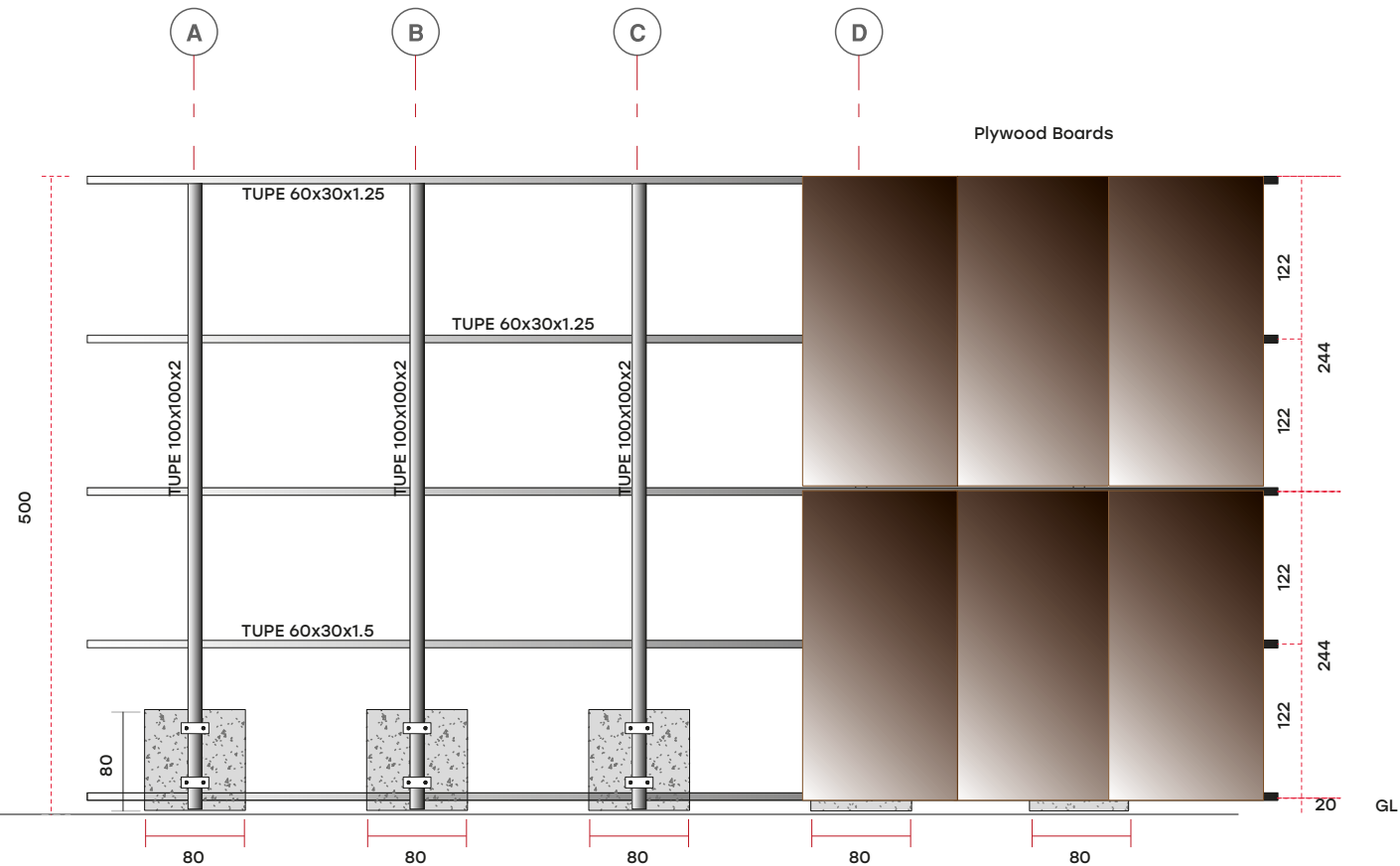
FRONT SIDE ELEVATION
