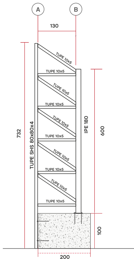
SIDE ELEVATION
