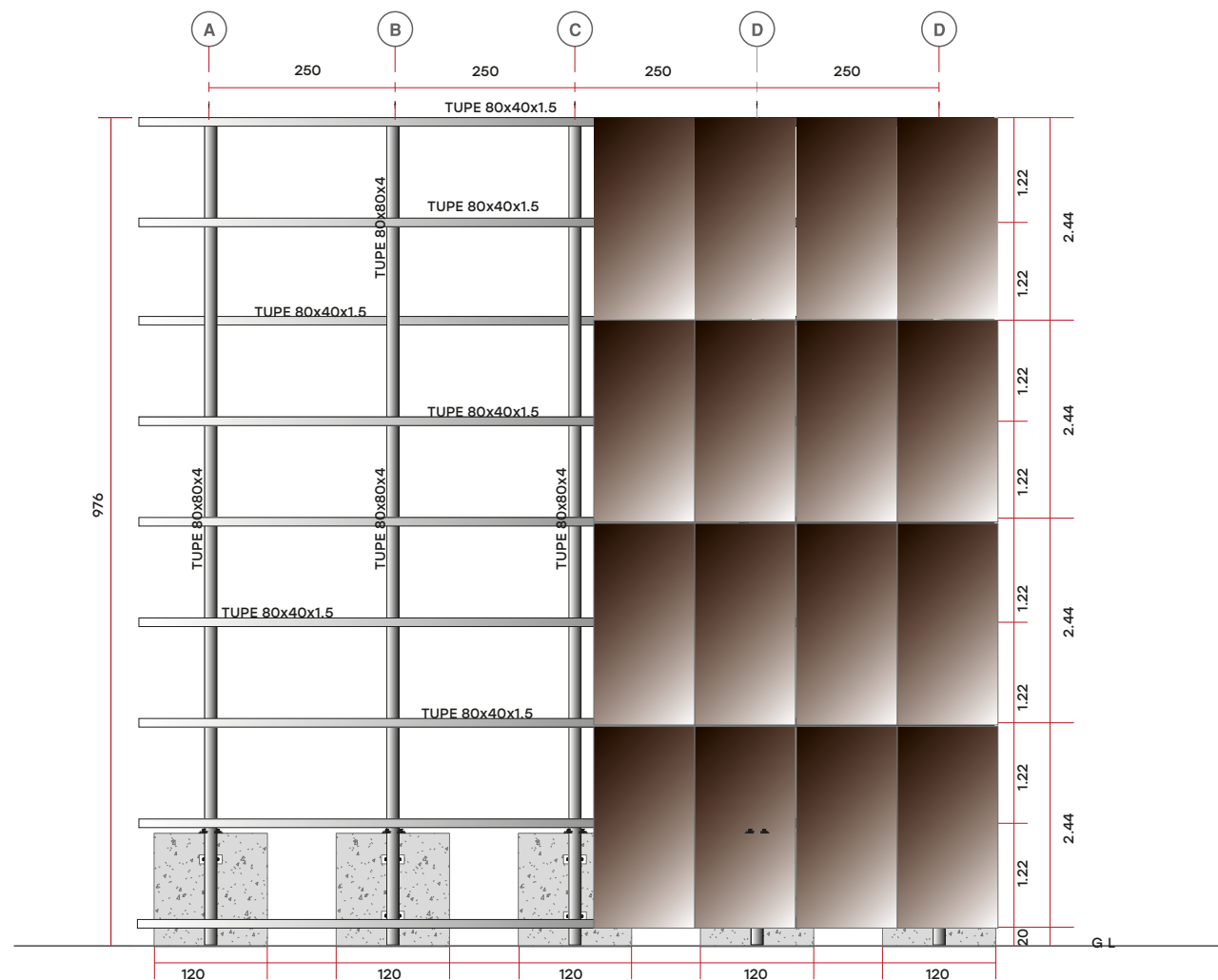
FRONT SIDE ELEVATION
