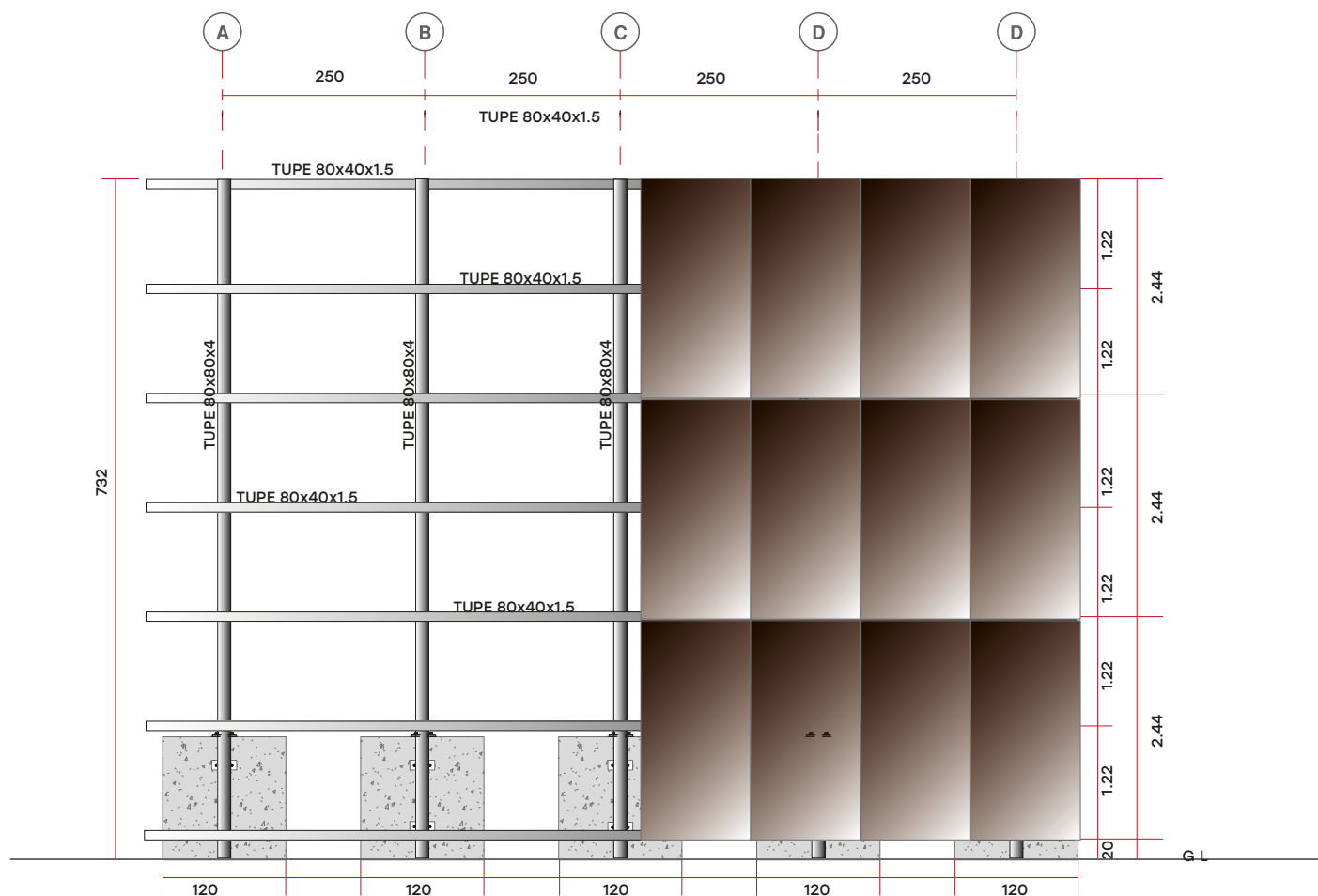
FRONT SIDE ELEVATION
