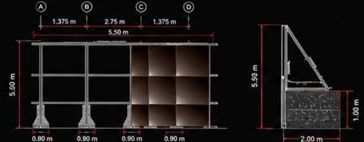
FRONT SIDE ELEVATION
