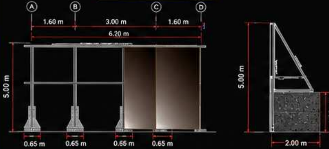
FRONT SIDE ELEVATION
