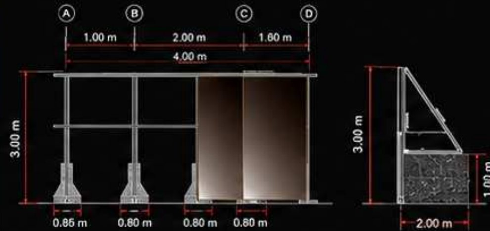
FRONT SIDE ELEVATION
